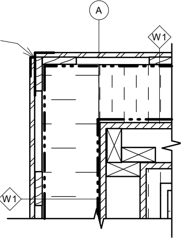
2 PLAN DETAIL - FLASHING DETAIL 1 : 10
