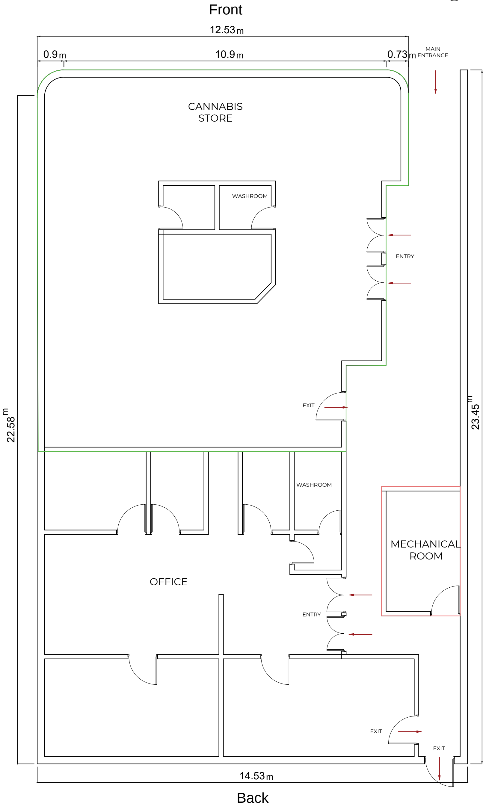
FLOOR PLAN
