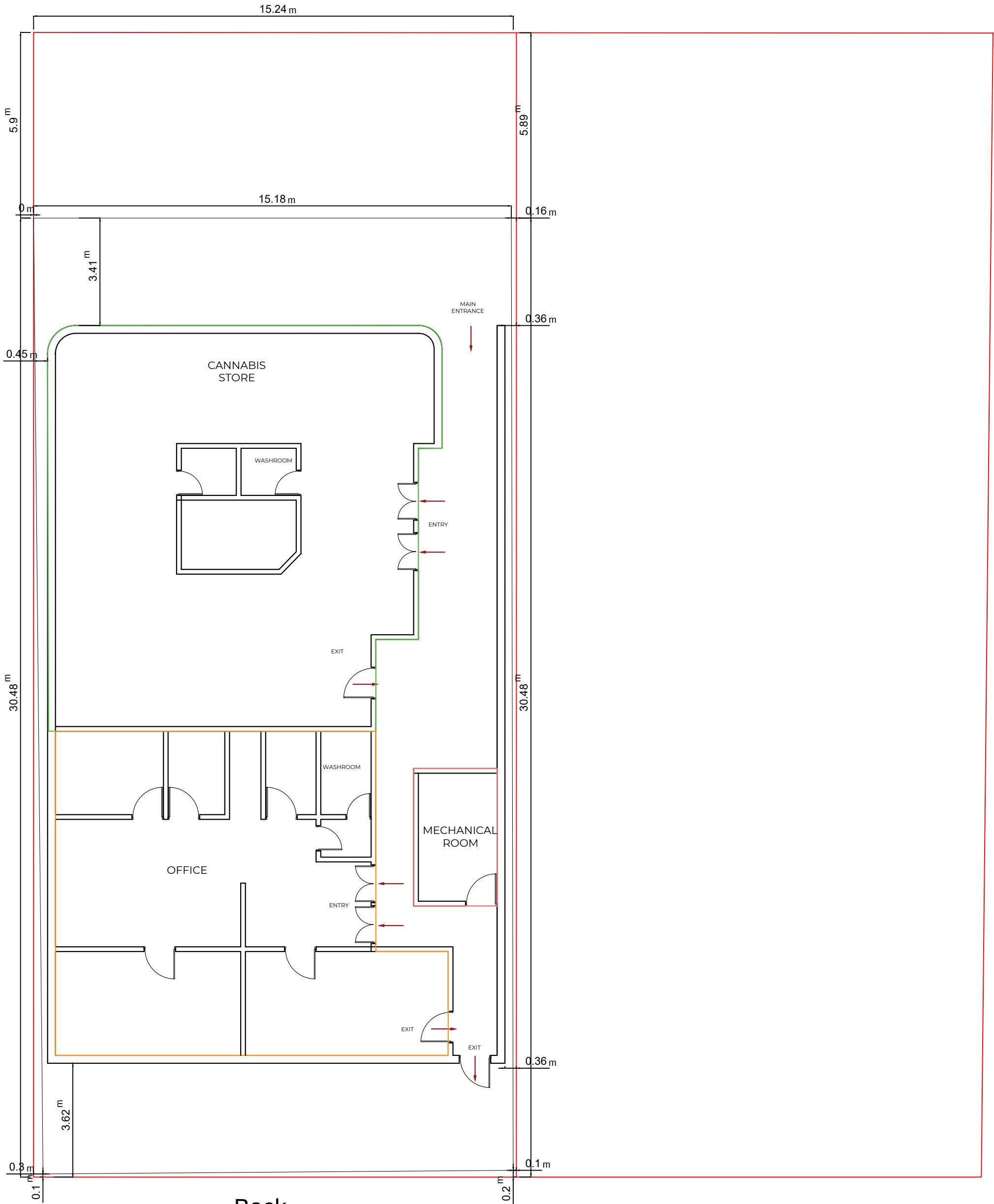
SETBACK DRAWING
