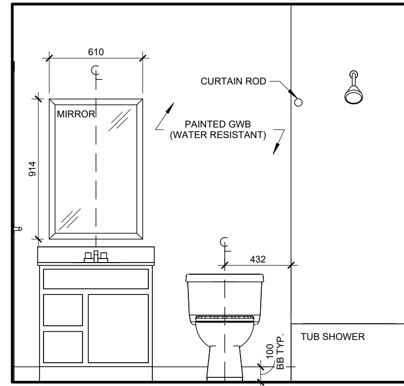
2 BATHROOM - INTERIOR ELEVATION 1 : 25
