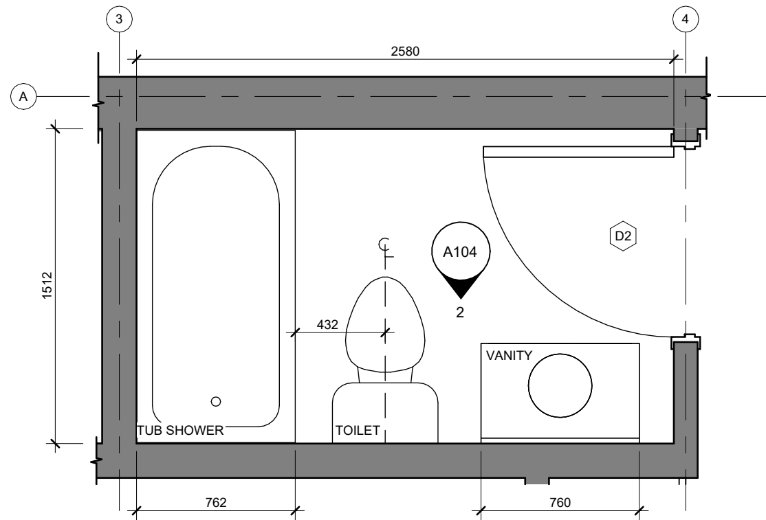
1 PARTIAL PLAN - BATHROOM TYP. 1 : 25
