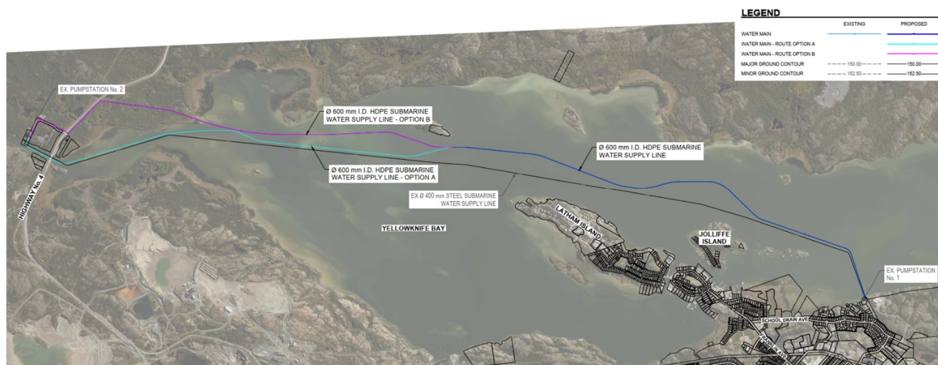
Figure 4-4: Pipeline from Pumphouse 2 to Pumphouse 1
